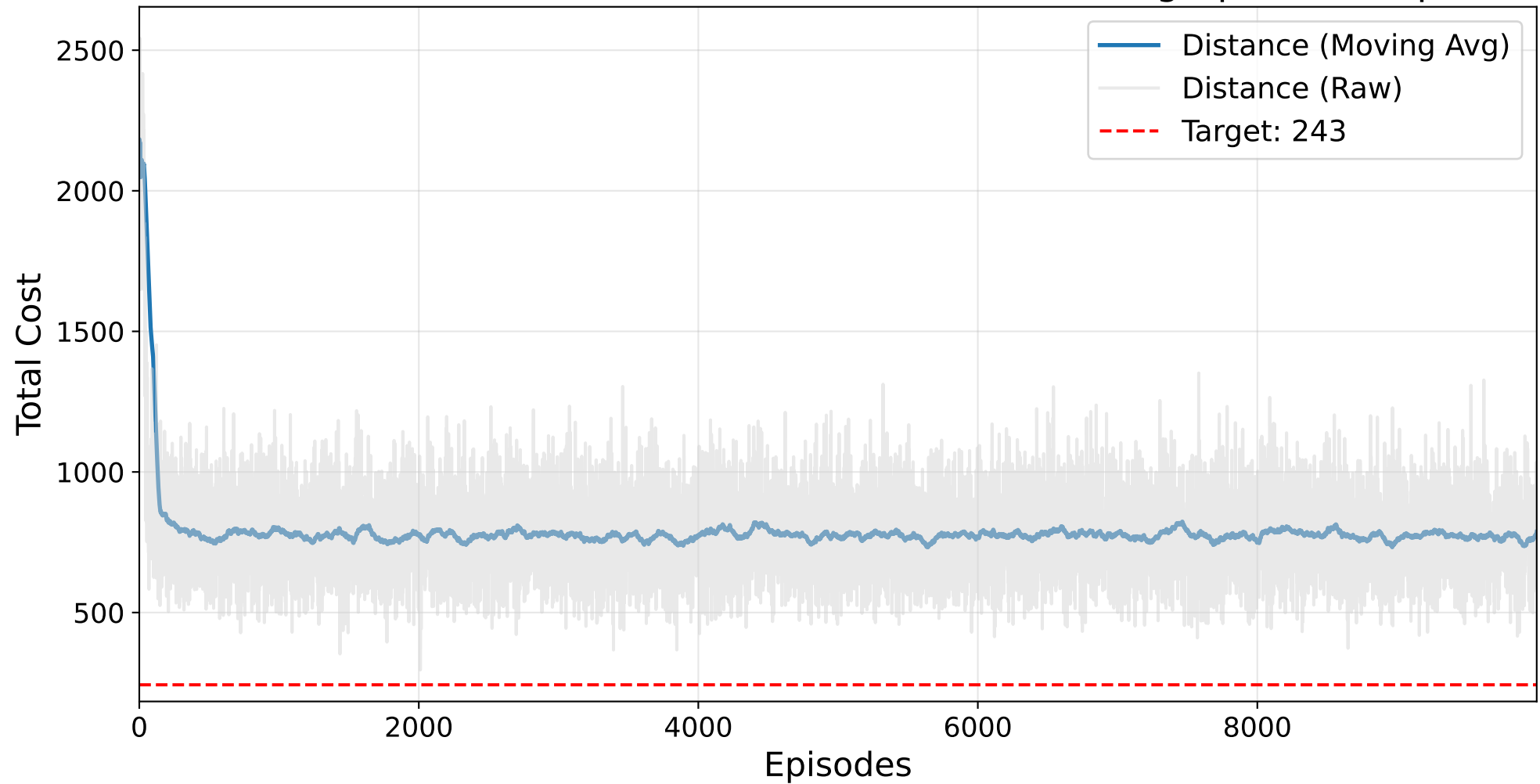
Final HYPERBAND GP Masked AutoRL-SOP Training - prob.42.sop
